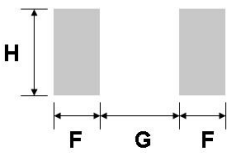
推荐焊盘设计 /Recommended pad layout
